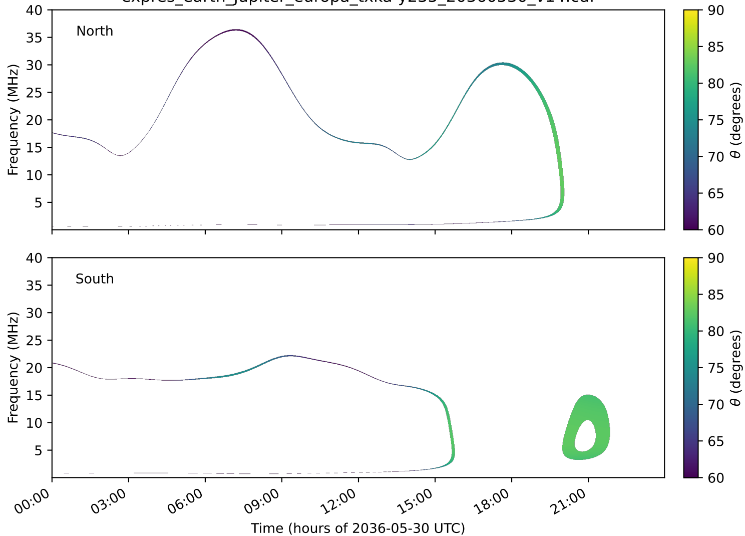
expres_earth_jupiter_europa_txka-y235_20360530_v14.cdf
