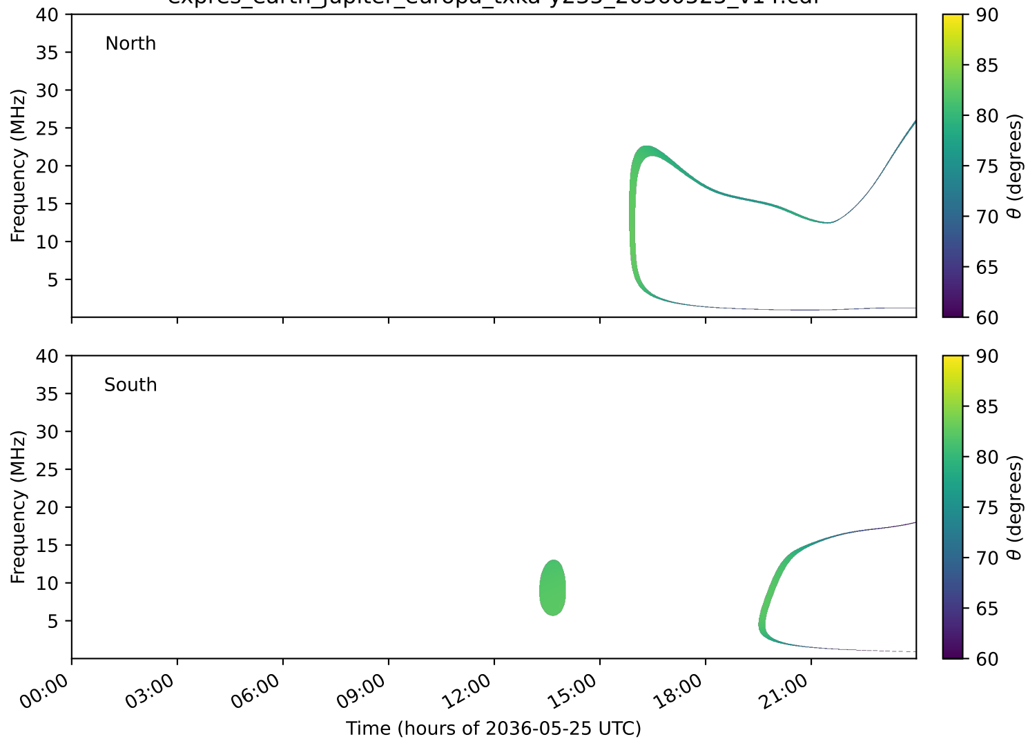
expres_earth_jupiter_europa_txka-y235_20360525_v14.cdf
