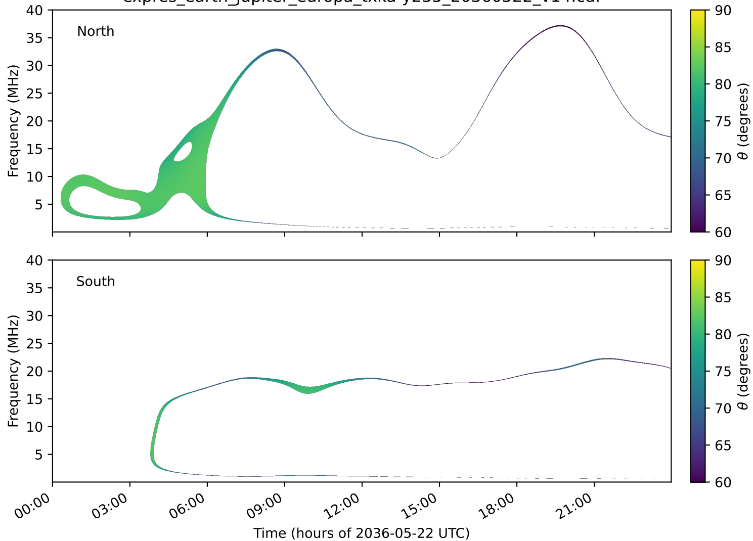
expres_earth_jupiter_europa_txka-y235_20360522_v14.cdf
