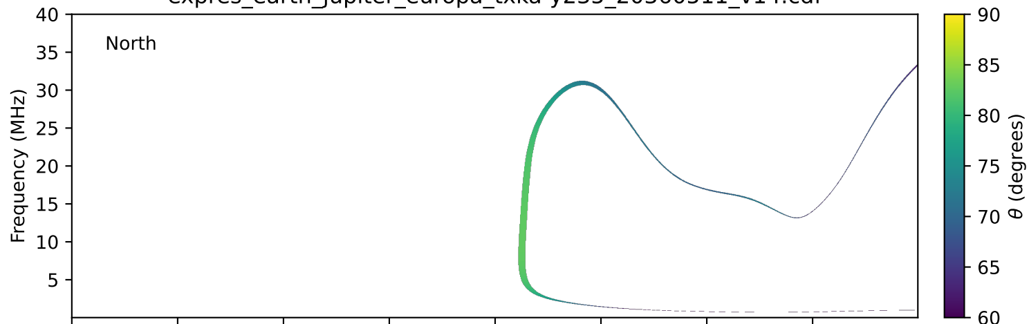
expres_earth_jupiter_europa_txka-y235_20360511_v14.cdf
