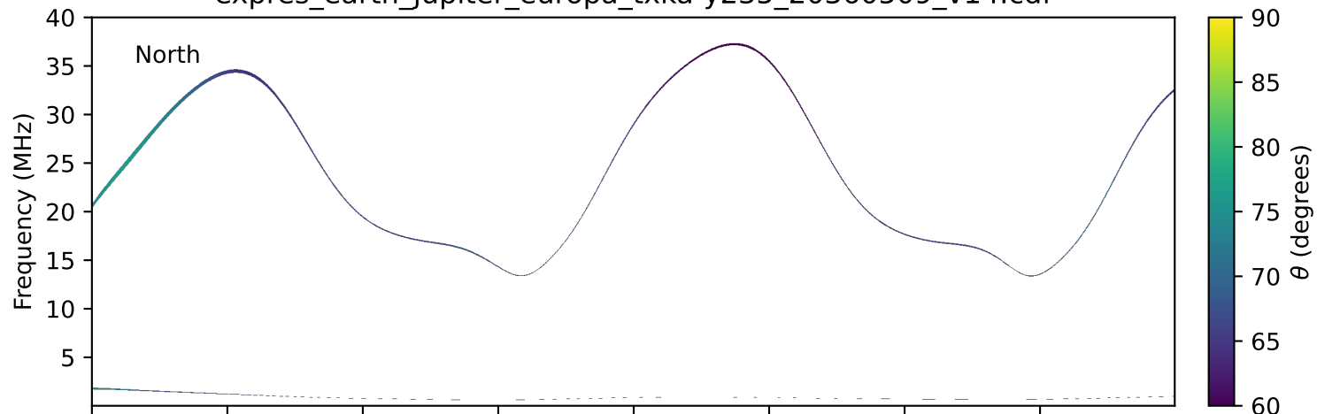
expres_earth_jupiter_europa_txka-y235_20360509_v14.cdf
