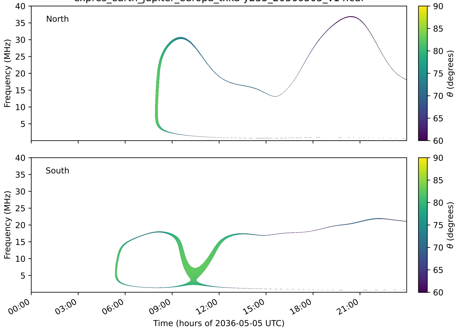
expres_earth_jupiter_europa_txka-y235_20360505_v14.cdf
