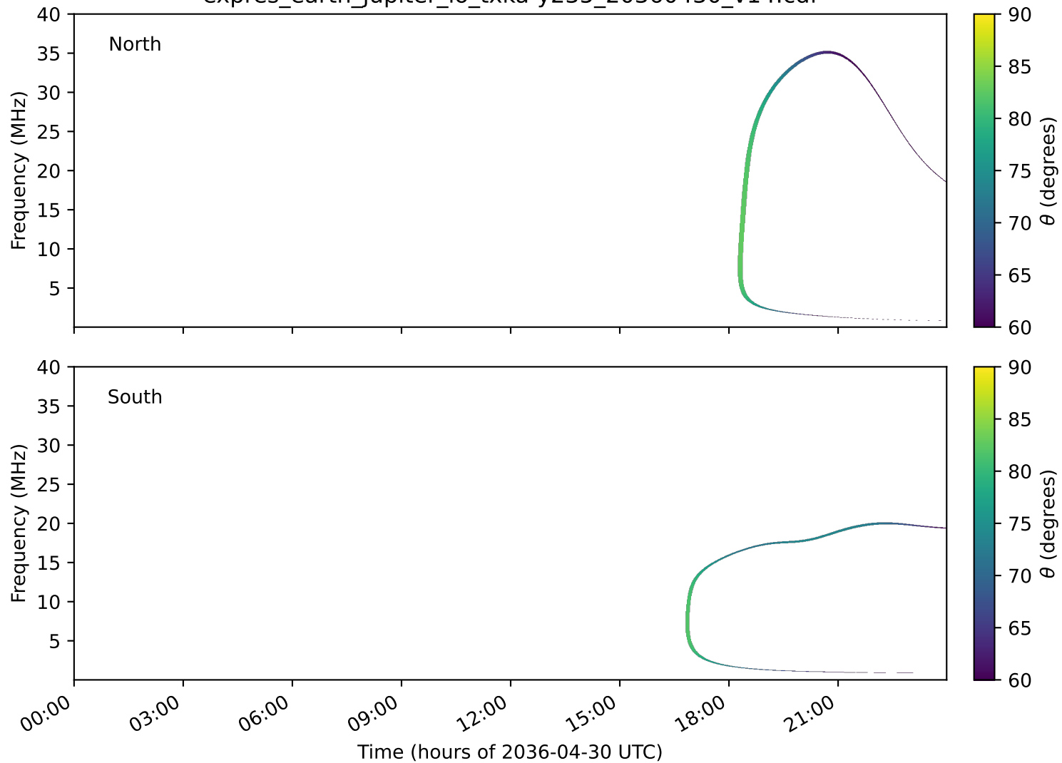
expres_earth_jupiter_io_txka-y235_20360430_v14.cdf
