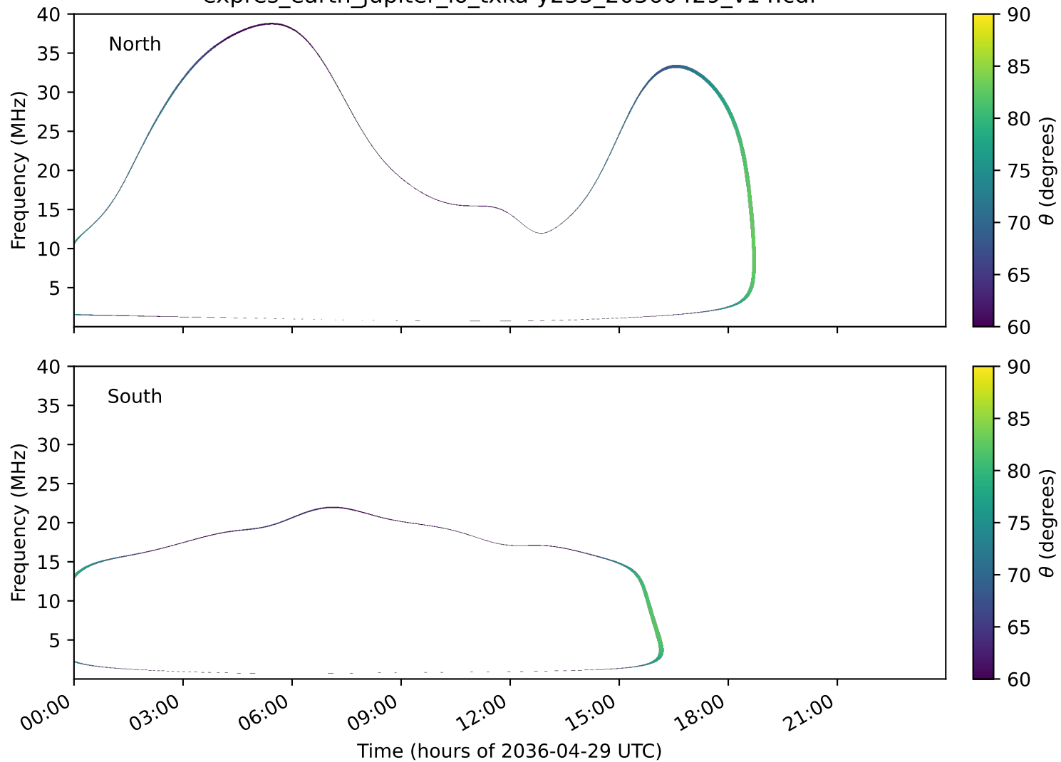
expres_earth_jupiter_io_txka-y235_20360429_v14.cdf
