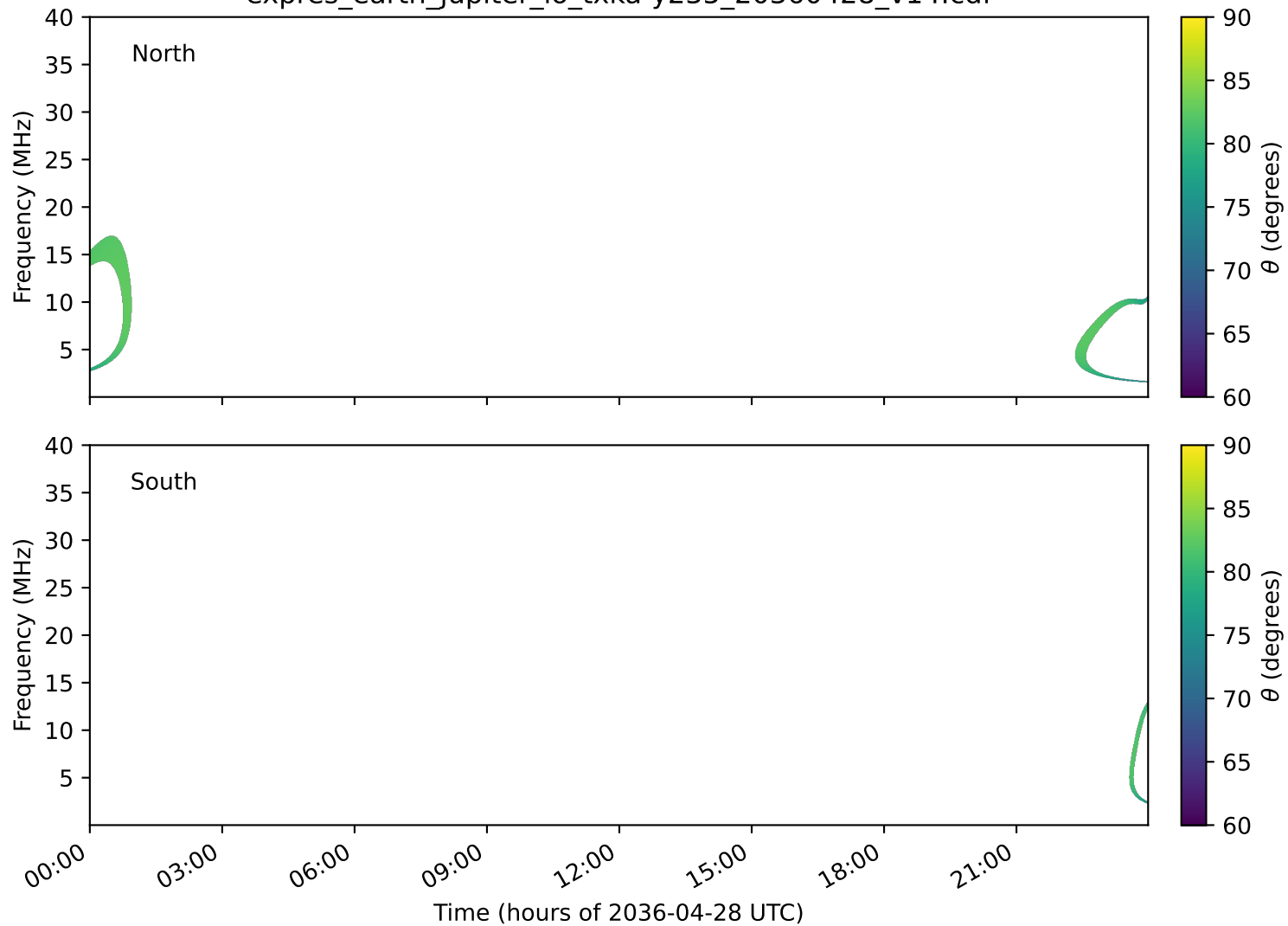
expres_earth_jupiter_io_txka-y235_20360428_v14.cdf
