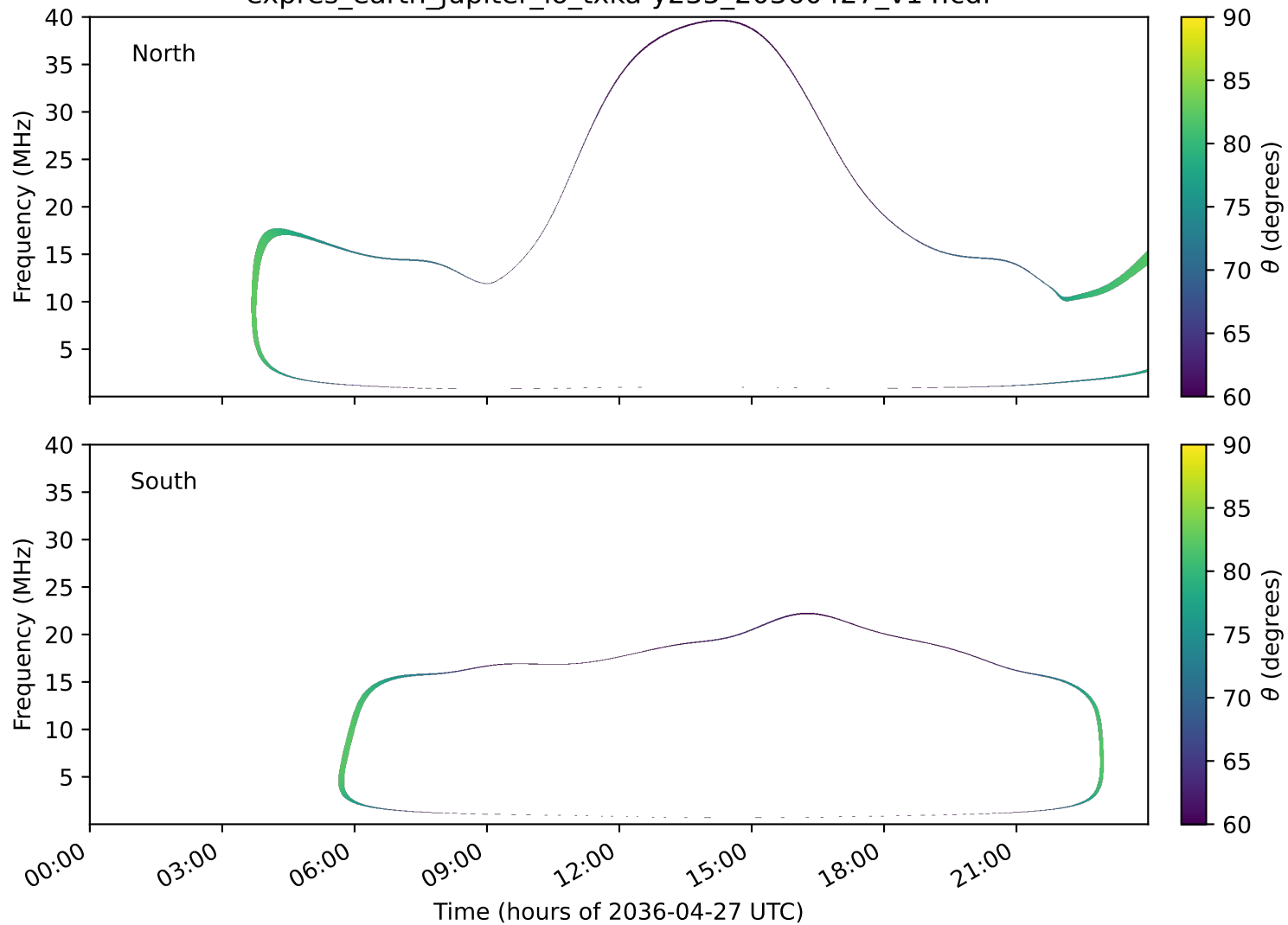
expres_earth_jupiter_io_txka-y235_20360427_v14.cdf
