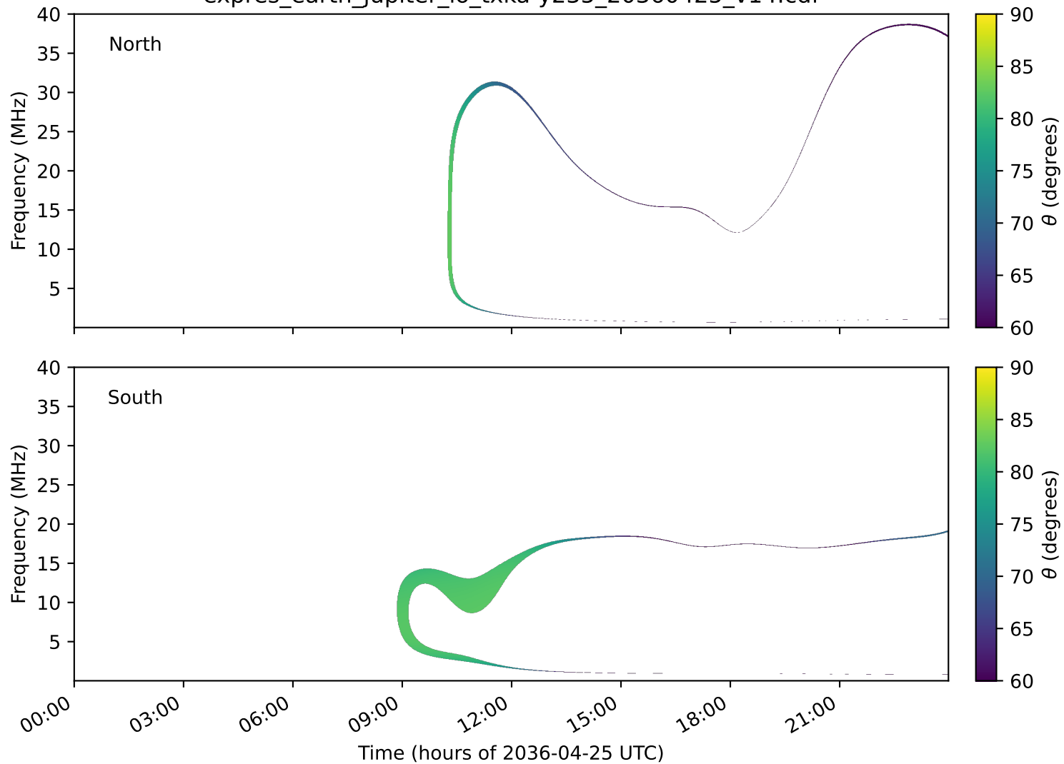
expres_earth_jupiter_io_txka-y235_20360425_v14.cdf
