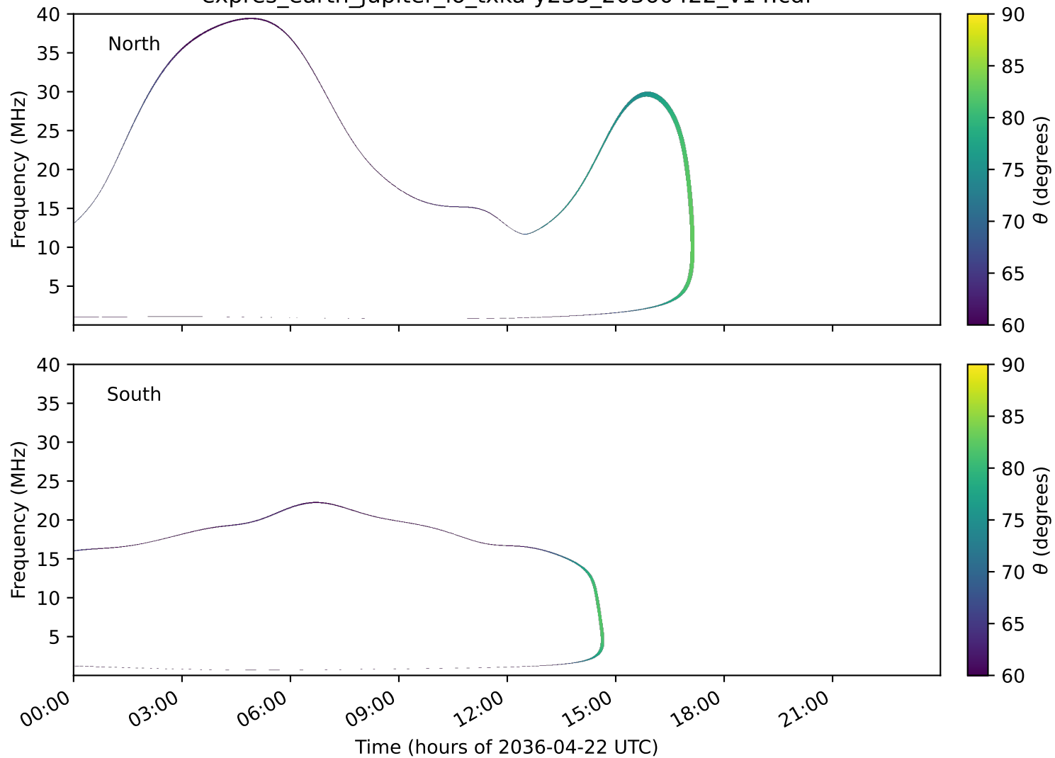
expres_earth_jupiter_io_txka-y235_20360422_v14.cdf
