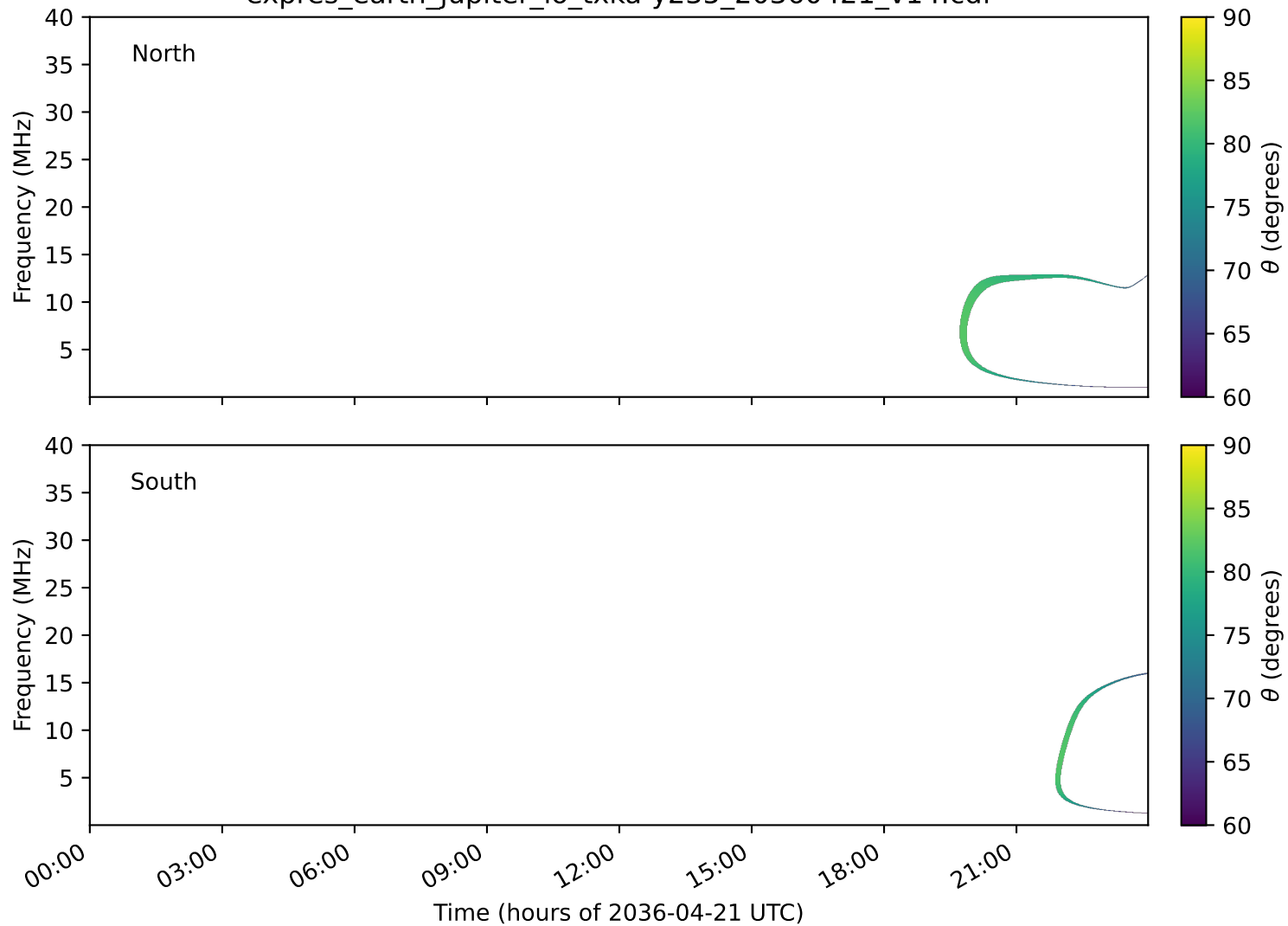
expres_earth_jupiter_io_txka-y235_20360421_v14.cdf
