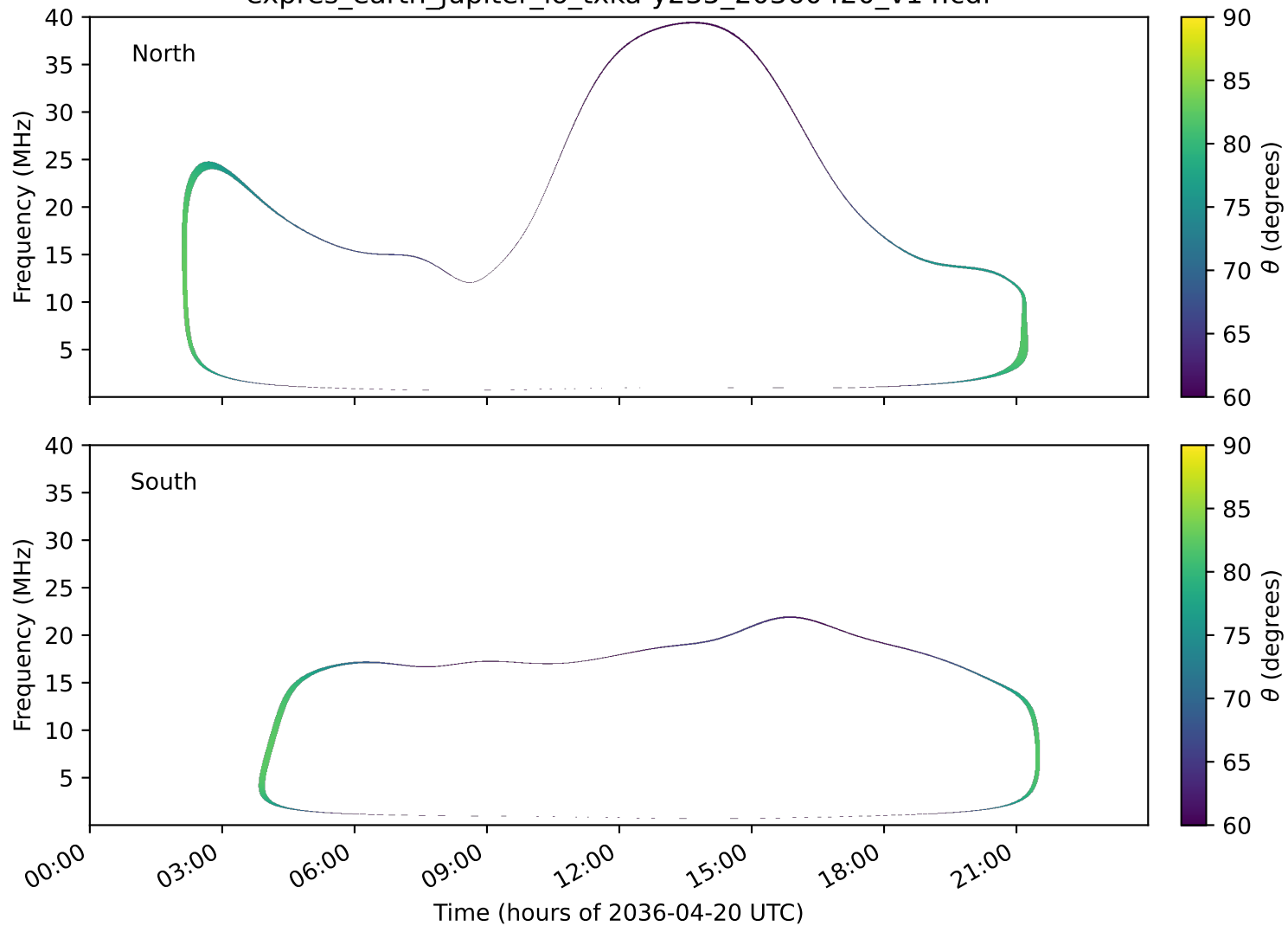
expres_earth_jupiter_io_txka-y235_20360420_v14.cdf
