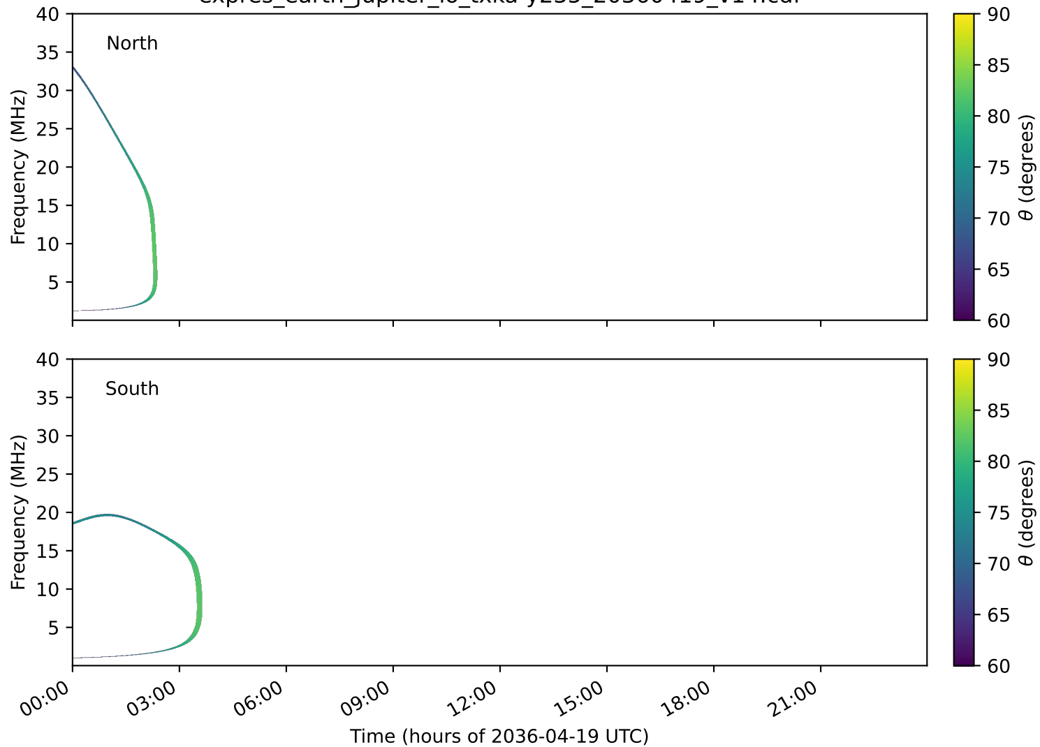
expres_earth_jupiter_io_txka-y235_20360419_v14.cdf
