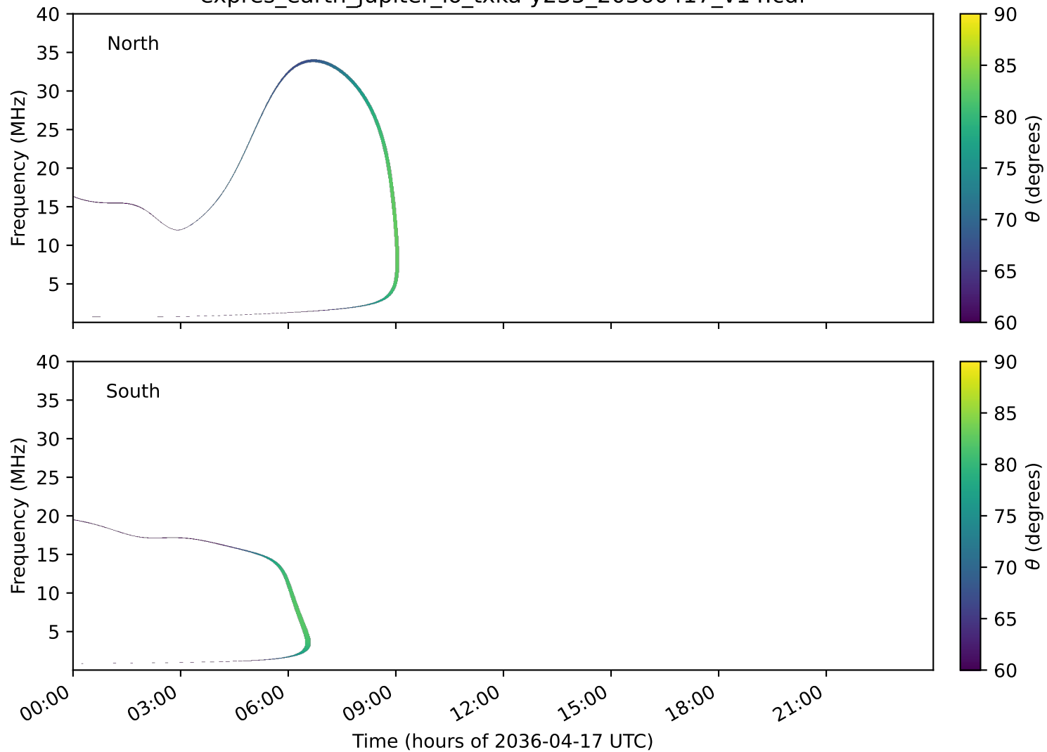
expres_earth_jupiter_io_txka-y235_20360417_v14.cdf
