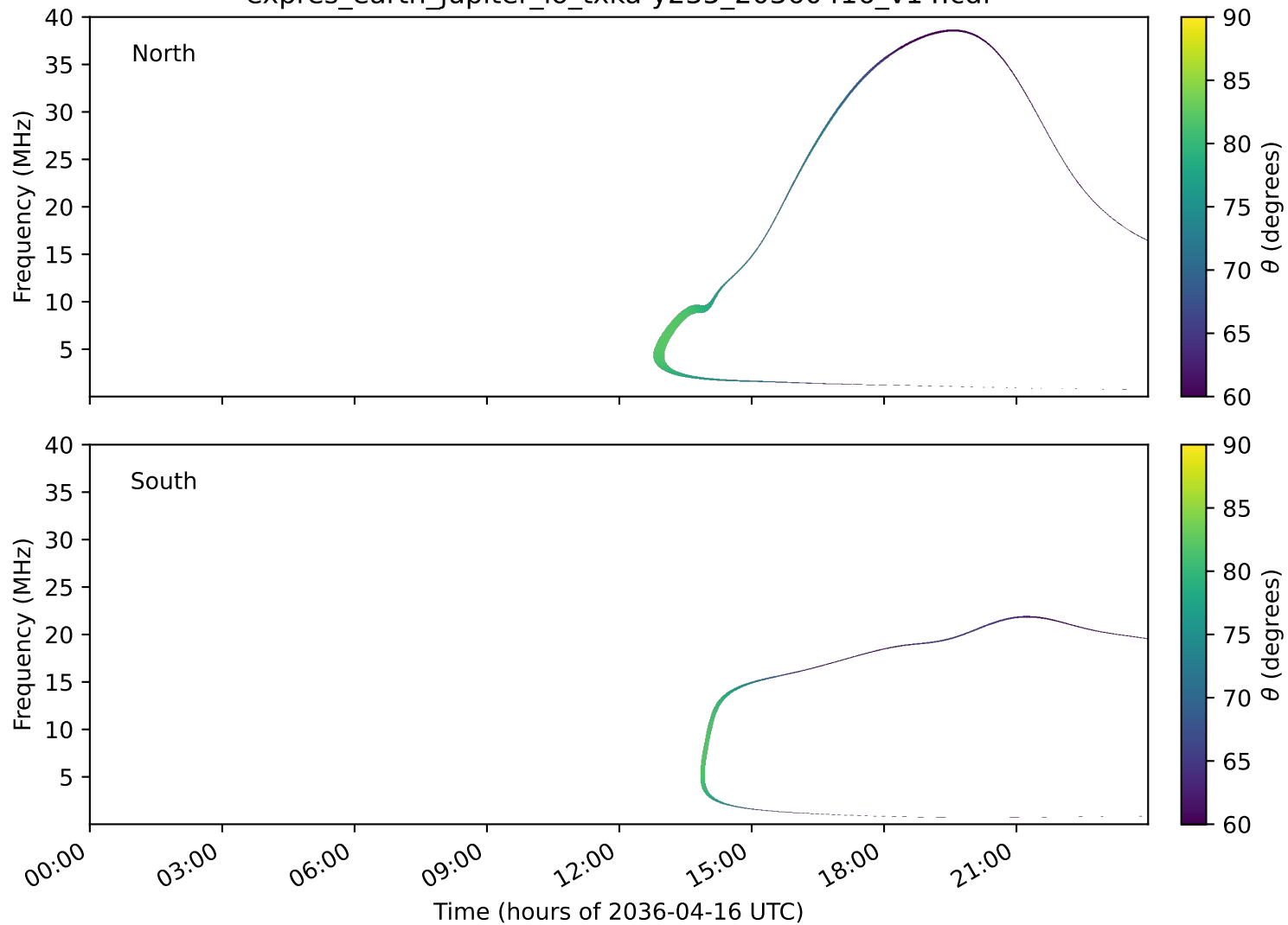
expres_earth_jupiter_io_txka-y235_20360416_v14.cdf
