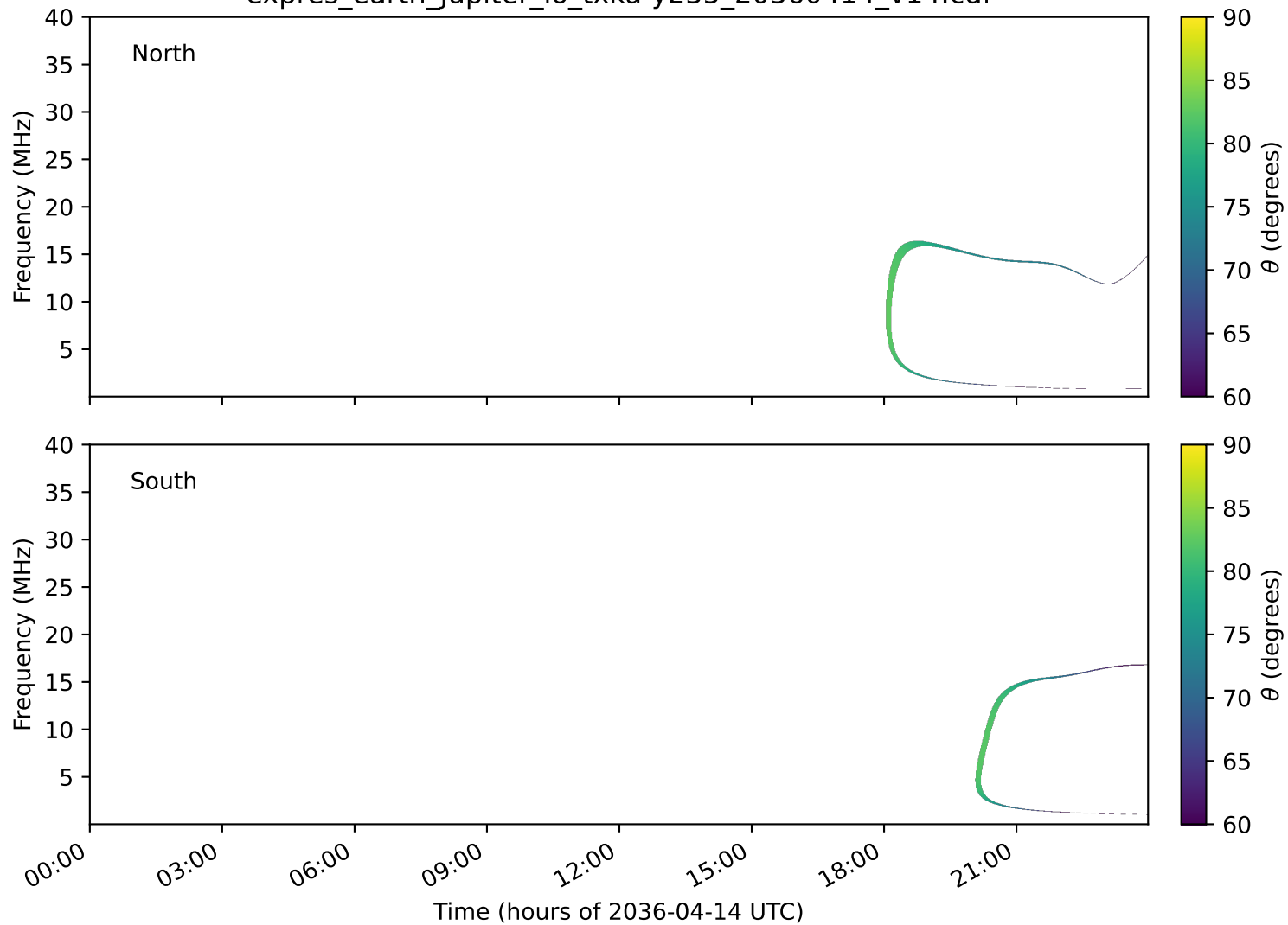
expres_earth_jupiter_io_txka-y235_20360414_v14.cdf
