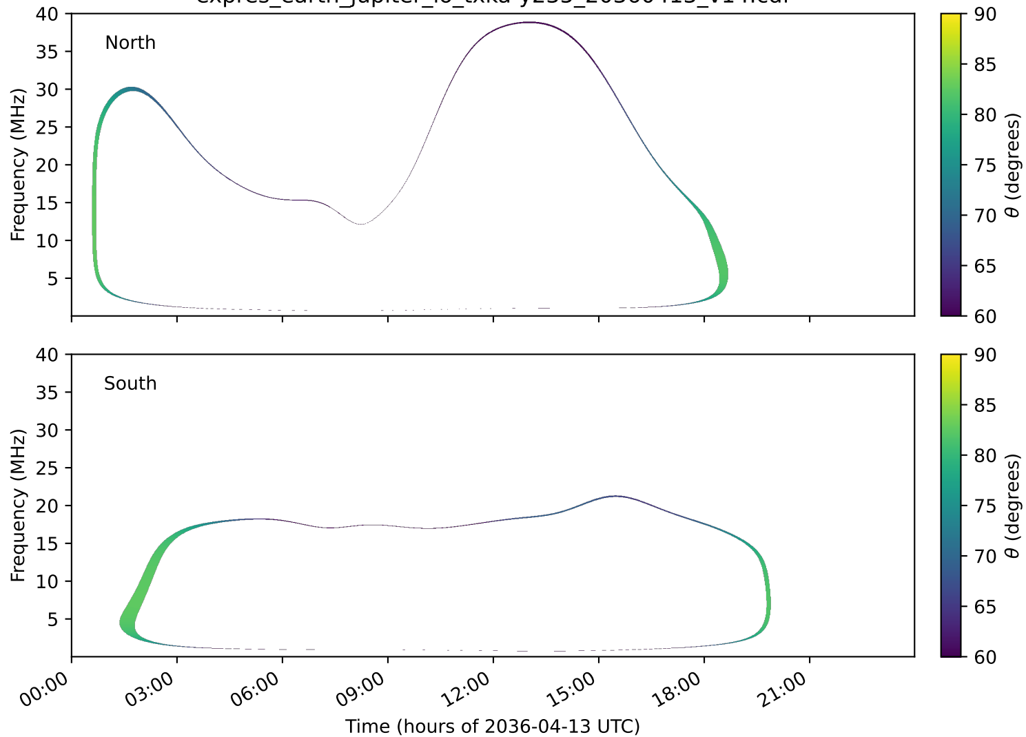
expres_earth_jupiter_io_txka-y235_20360413_v14.cdf
