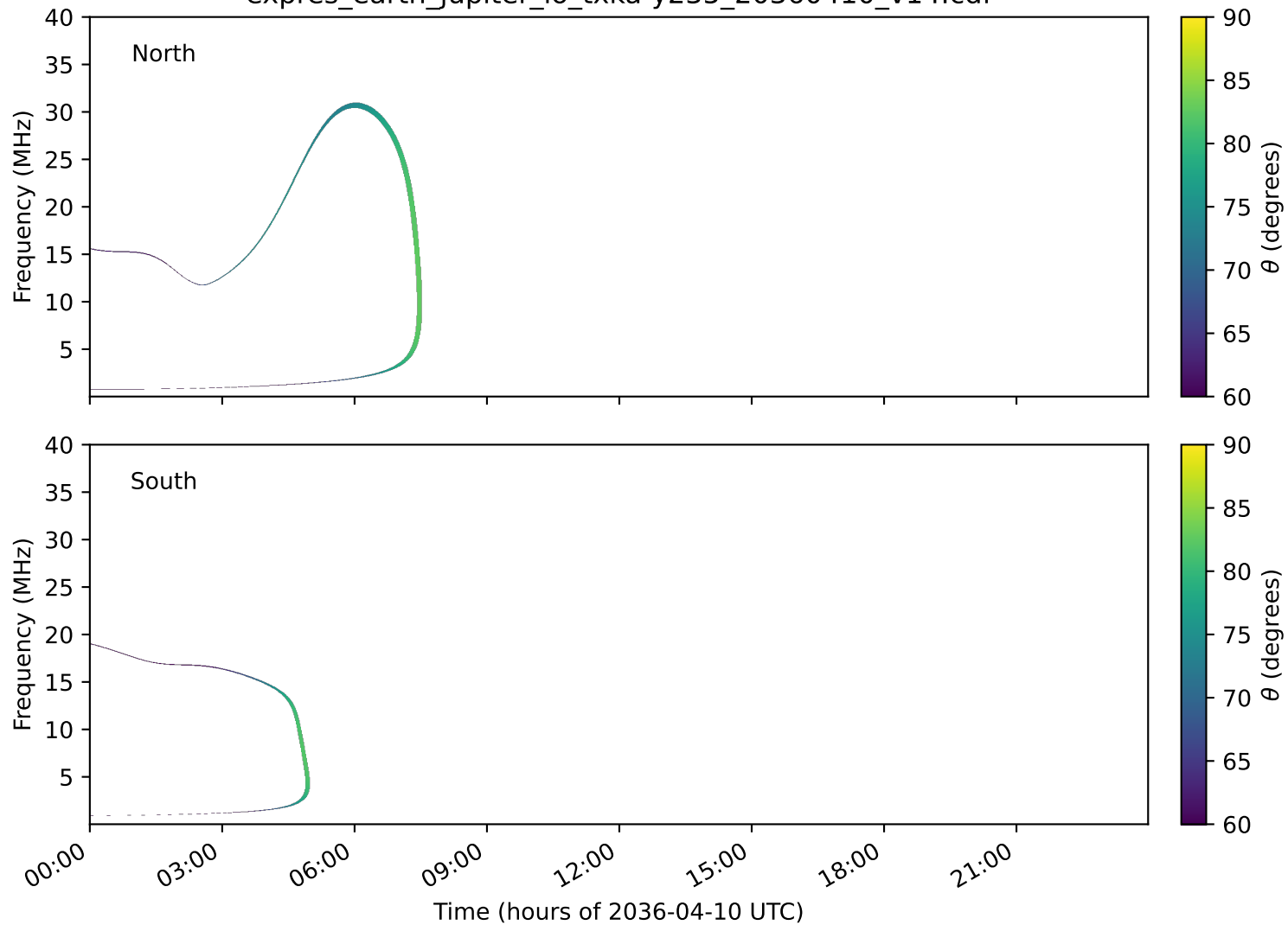
expres_earth_jupiter_io_txka-y235_20360410_v14.cdf
