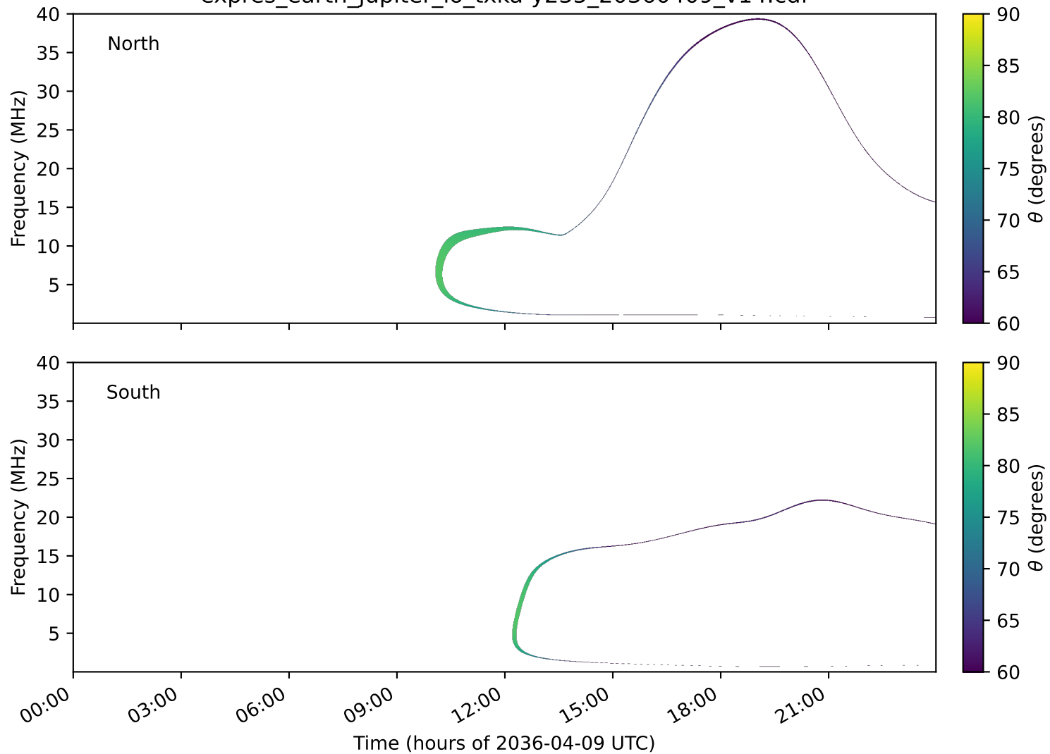
expres_earth_jupiter_io_txka-y235_20360409_v14.cdf
