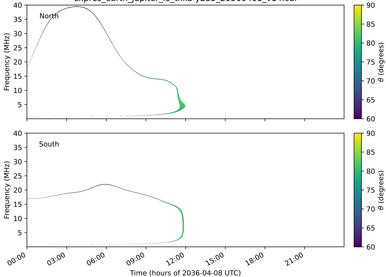
expres_earth_jupiter_io_txka-y235_20360408_v14.cdf
