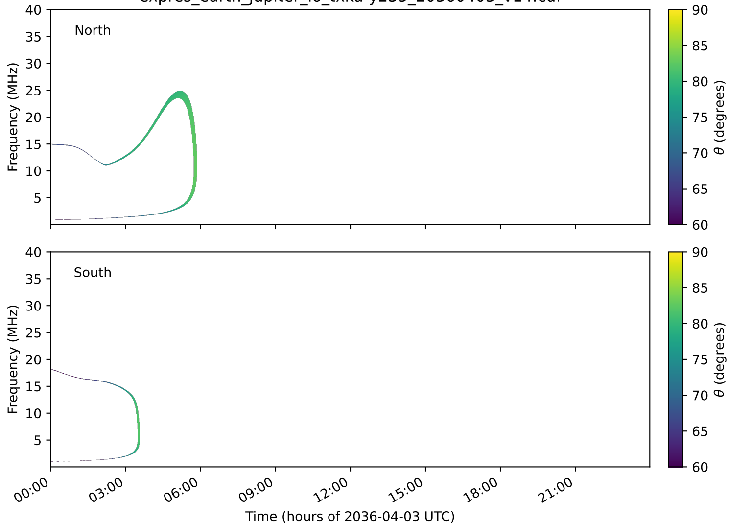
expres_earth_jupiter_io_txka-y235_20360403_v14.cdf
