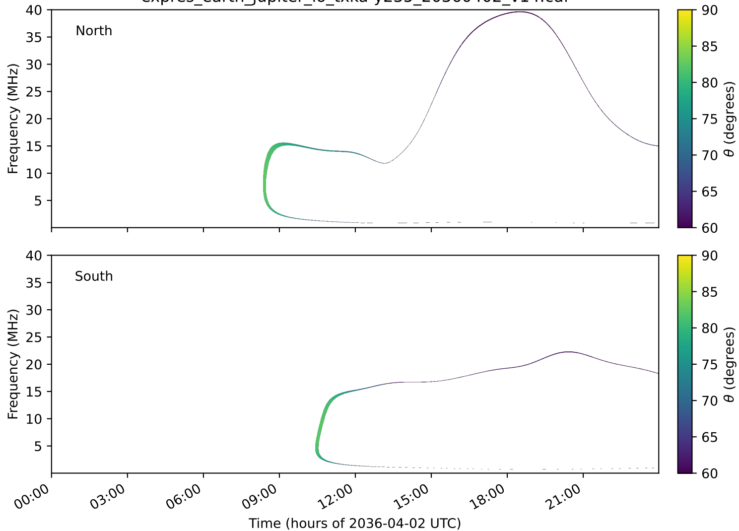
expres_earth_jupiter_io_txka-y235_20360402_v14.cdf
