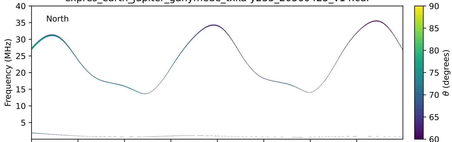
expres_earth_jupiter_ganymede_txka-y235_20360425_v14.cdf
