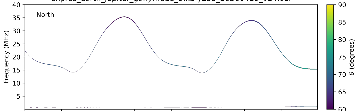
expres_earth_jupiter_ganymede_txka-y235_20360419_v14.cdf
