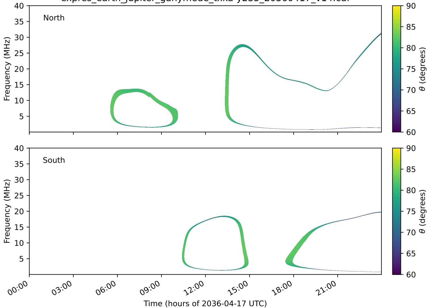
expres_earth_jupiter_ganymede_txka-y235_20360417_v14.cdf
