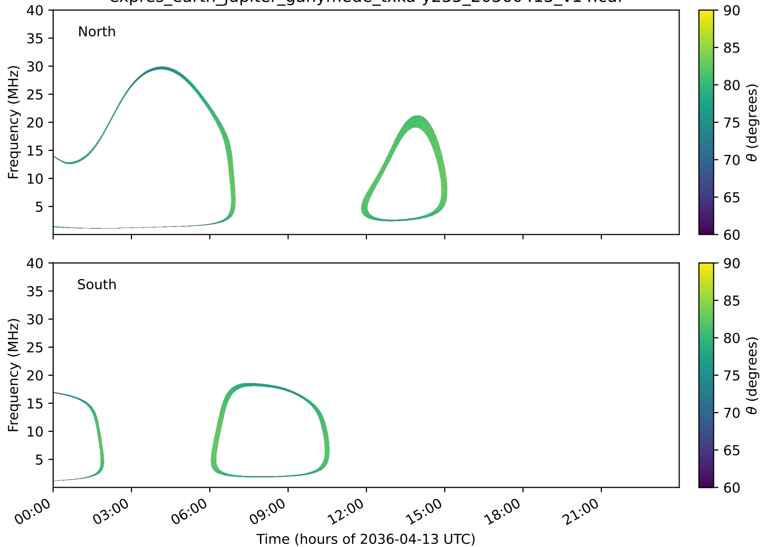
expres_earth_jupiter_ganymede_txka-y235_20360413_v14.cdf
