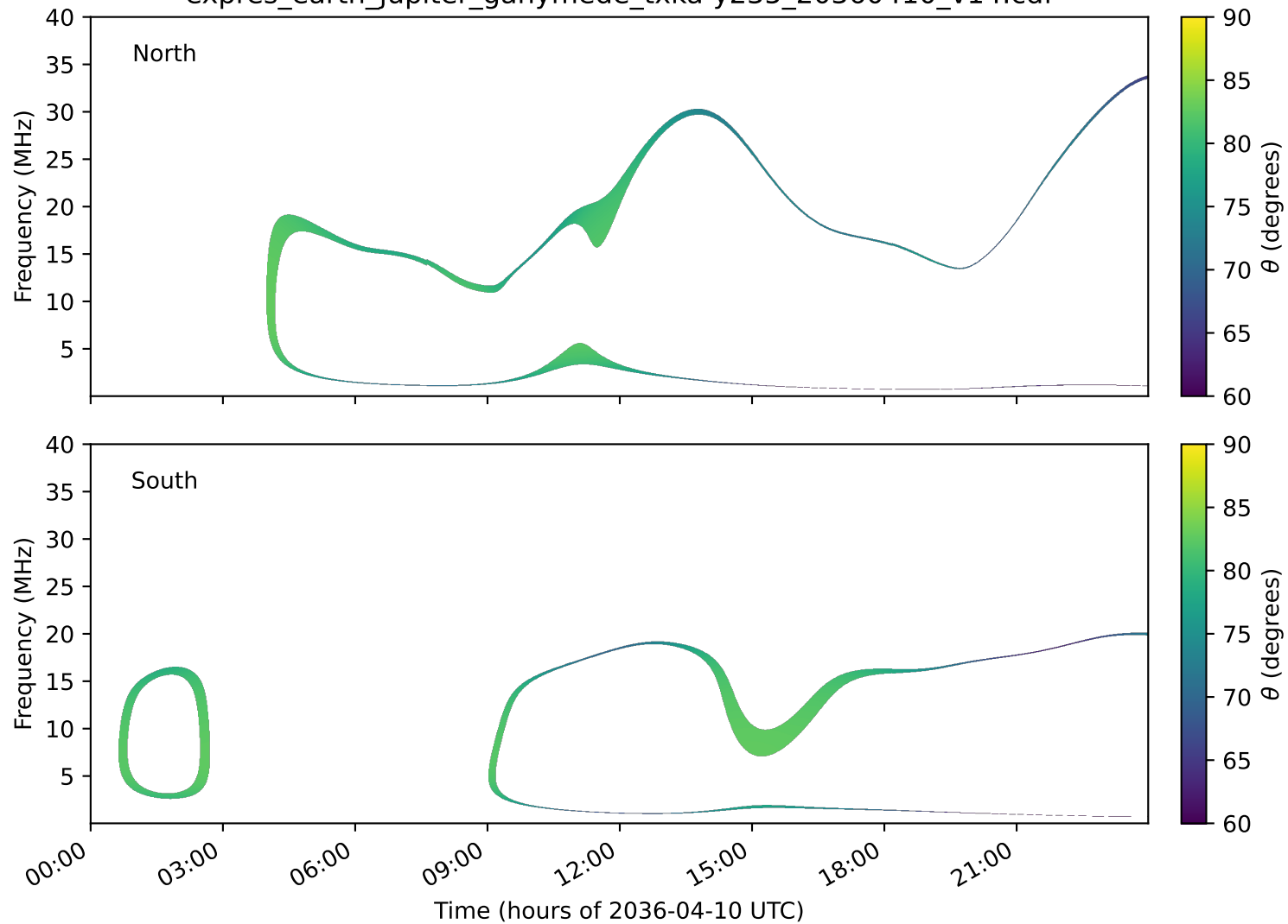
expres_earth_jupiter_ganymede_txka-y235_20360410_v14.cdf
