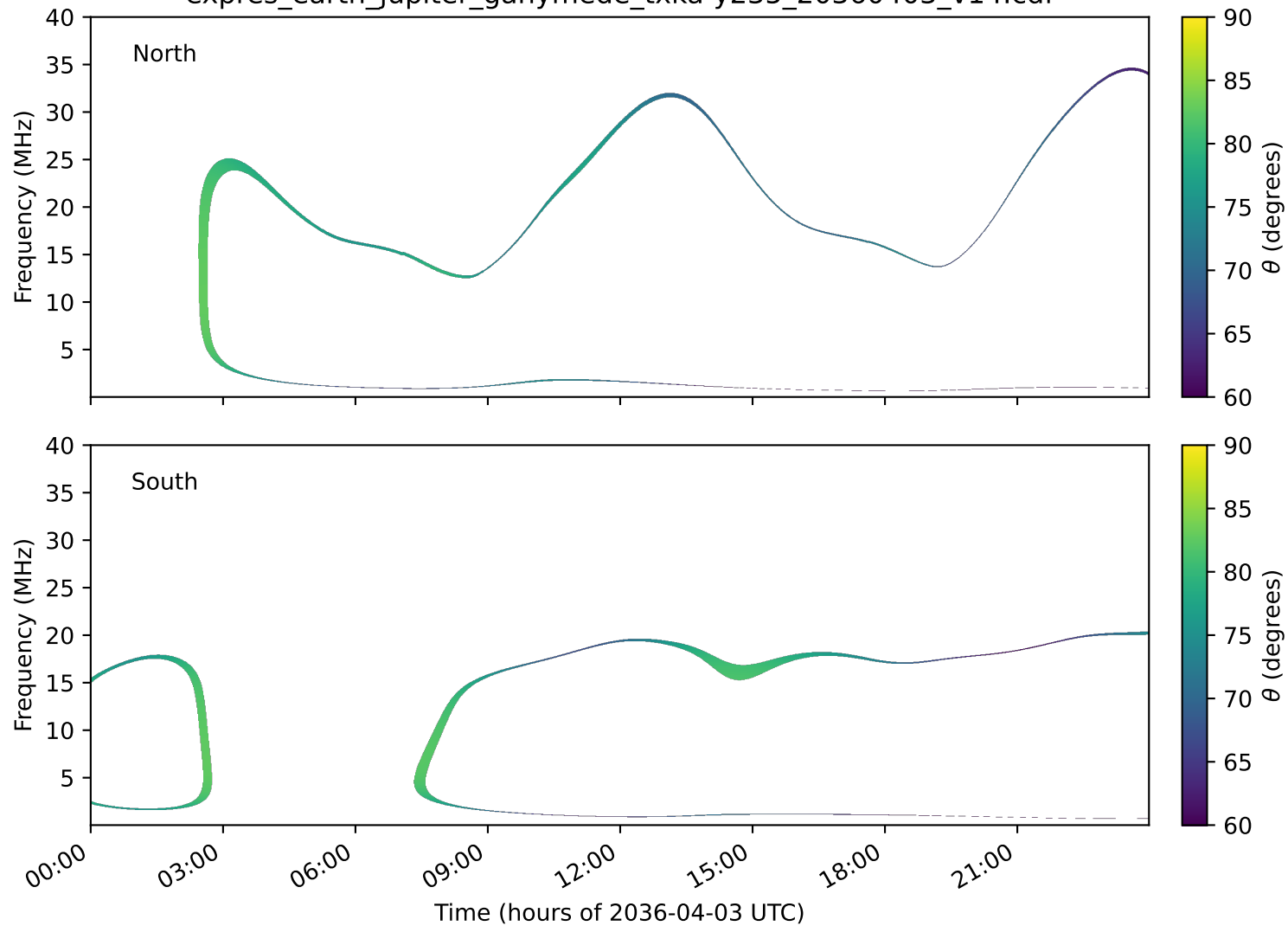
expres_earth_jupiter_ganymede_txka-y235_20360403_v14.cdf
