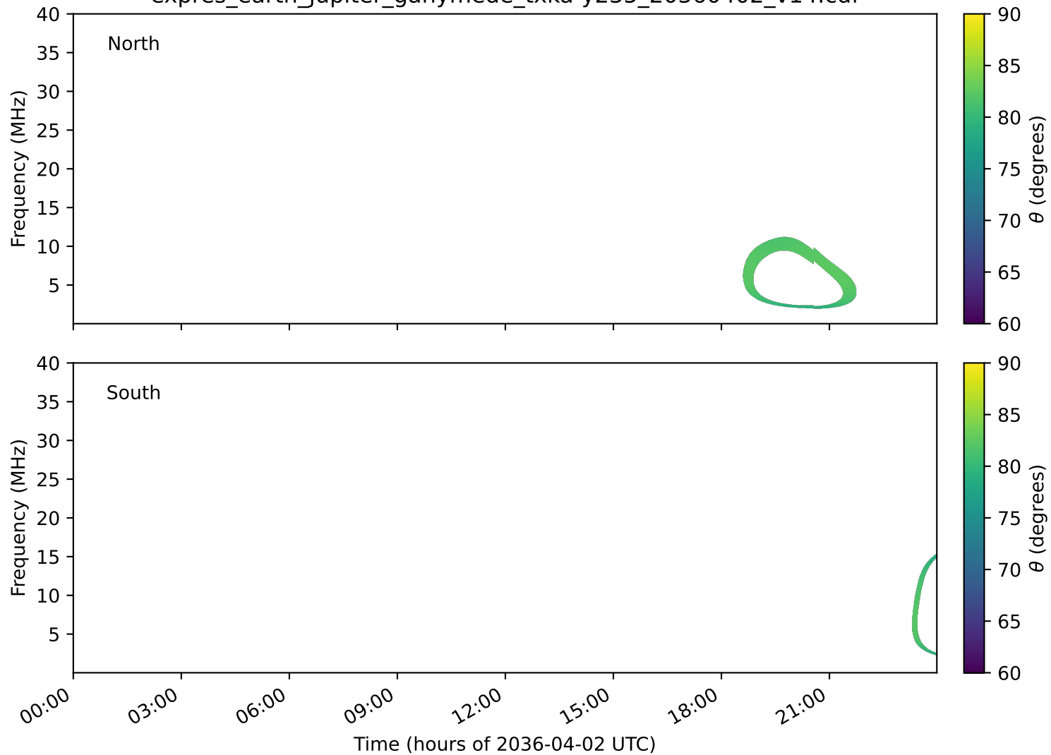
expres_earth_jupiter_ganymede_txka-y235_20360402_v14.cdf
