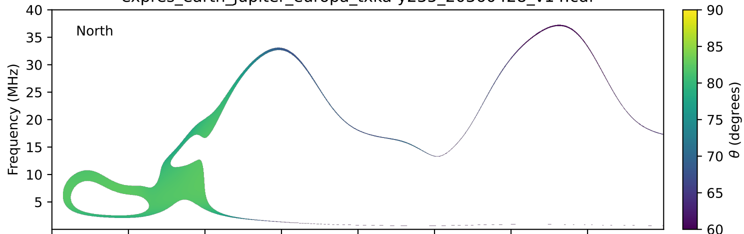
expres_earth_jupiter_europa_txka-y235_20360428_v14.cdf
