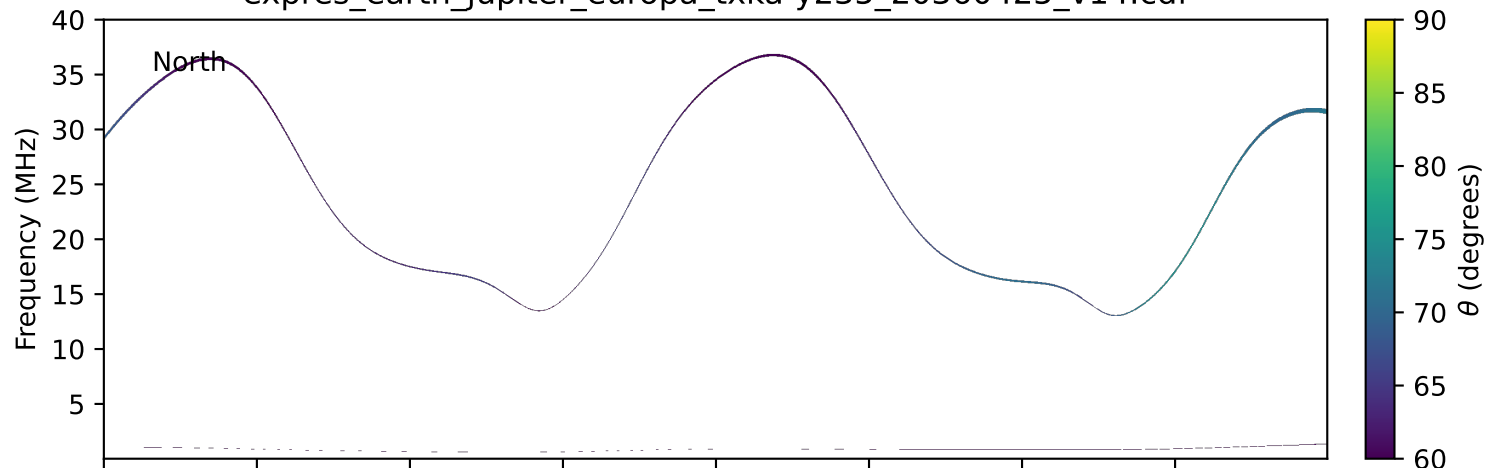
expres_earth_jupiter_europa_txka-y235_20360425_v14.cdf
