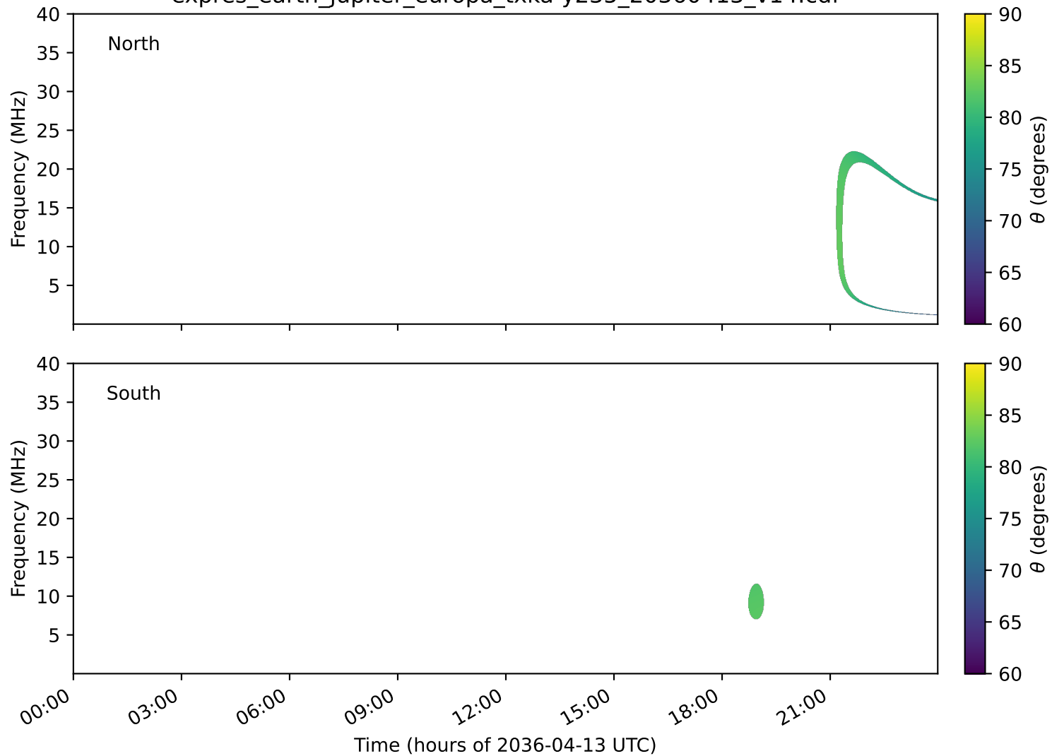
expres_earth_jupiter_europa_txka-y235_20360413_v14.cdf
