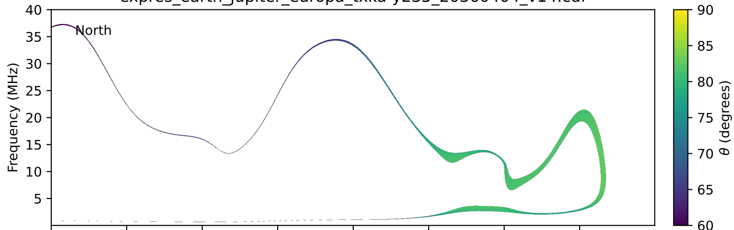
expres_earth_jupiter_europa_txka-y235_20360404_v14.cdf
