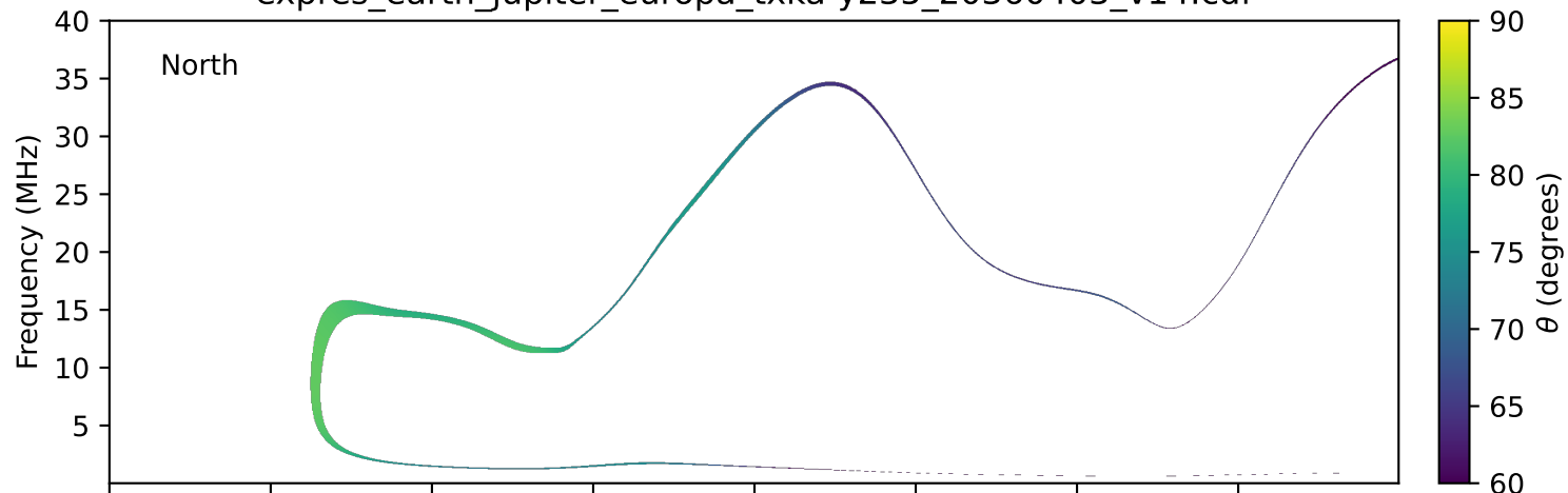
expres_earth_jupiter_europa_txka-y235_20360403_v14.cdf
