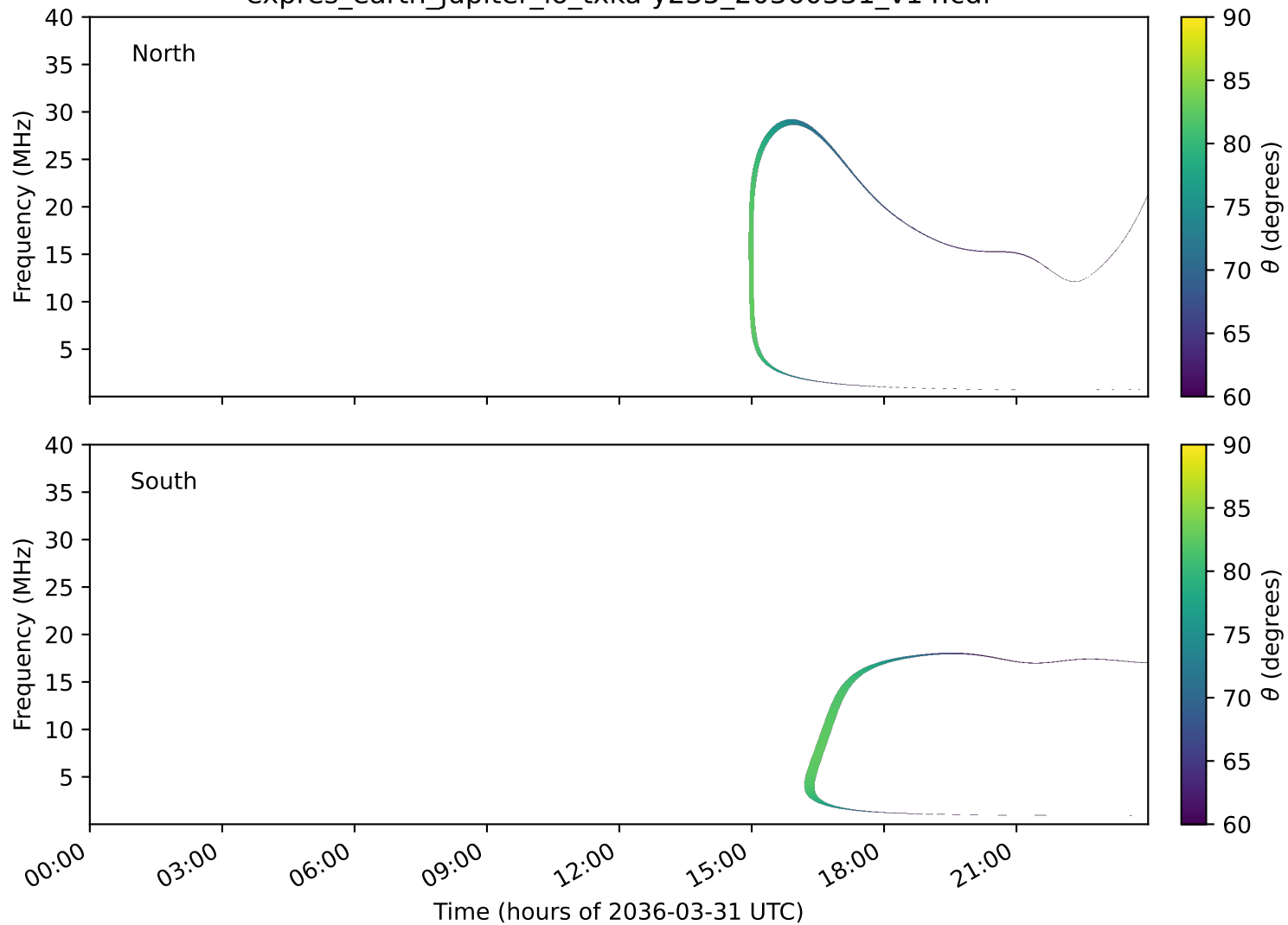
expres_earth_jupiter_io_txka-y235_20360331_v14.cdf
