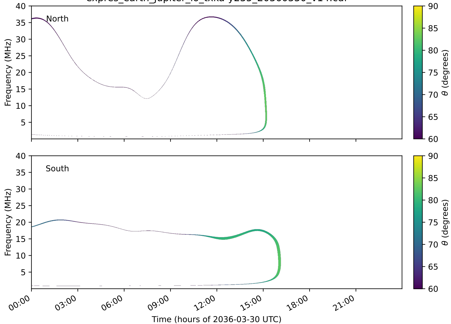
expres_earth_jupiter_io_txka-y235_20360330_v14.cdf
