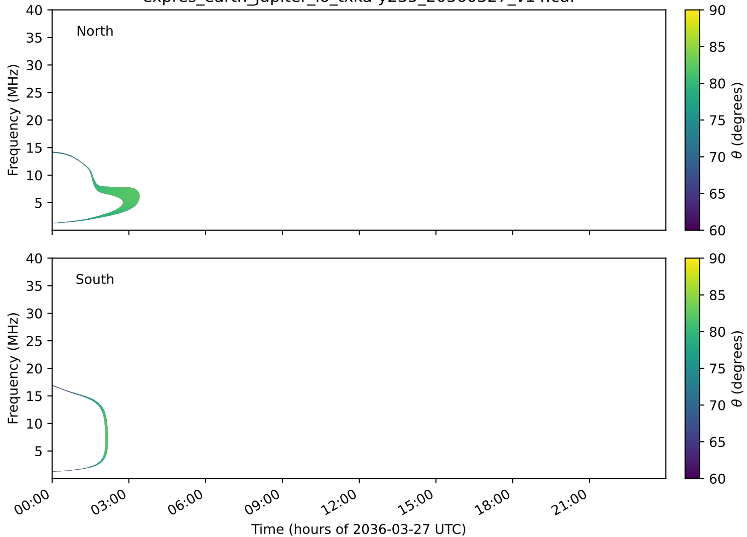
expres_earth_jupiter_io_txka-y235_20360327_v14.cdf
