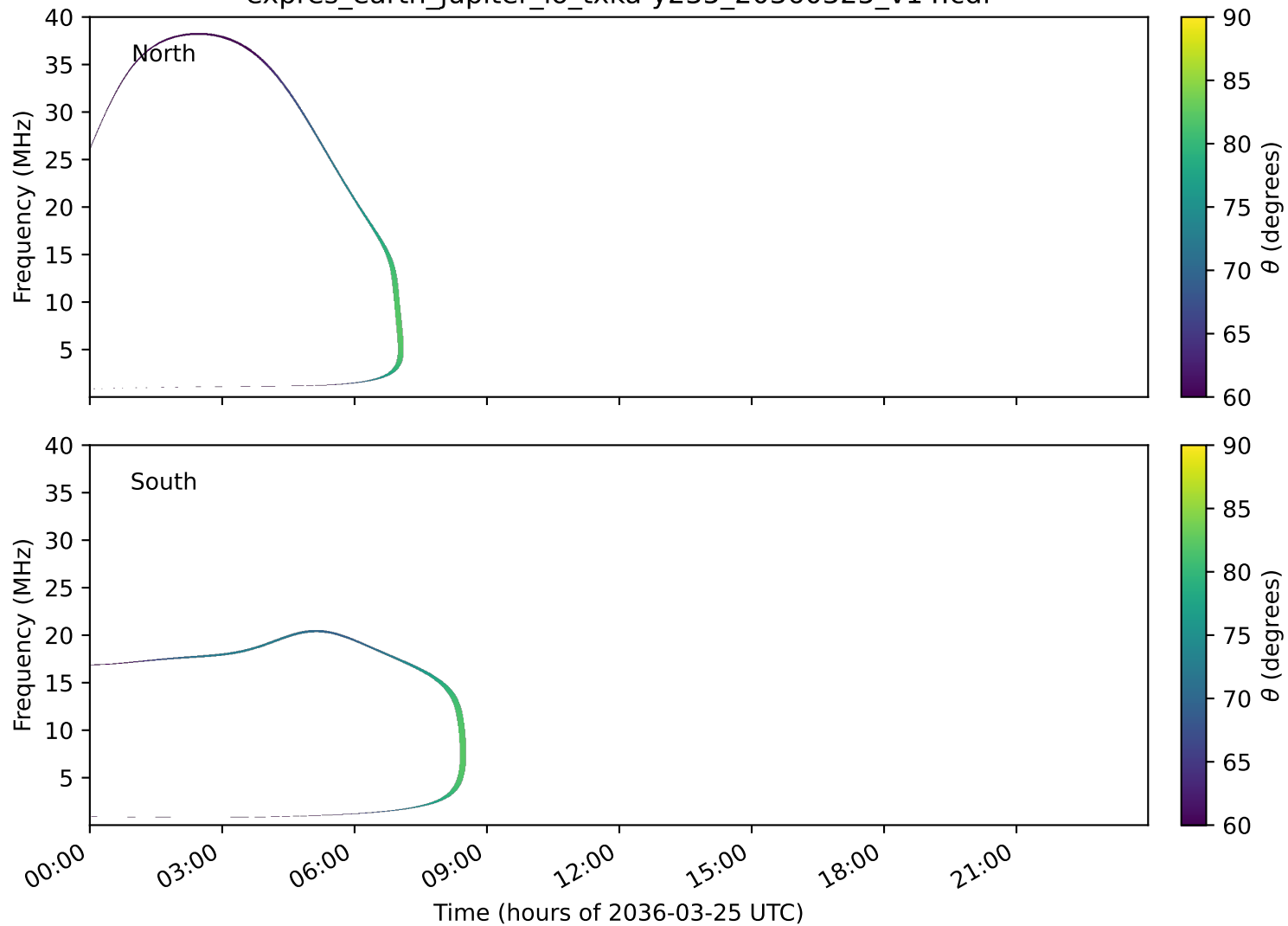
expres_earth_jupiter_io_txka-y235_20360325_v14.cdf
