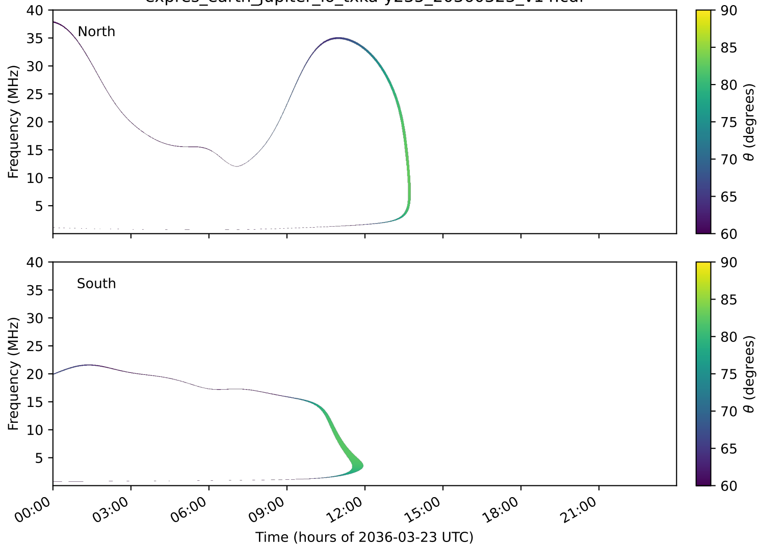
expres_earth_jupiter_io_txka-y235_20360323_v14.cdf
