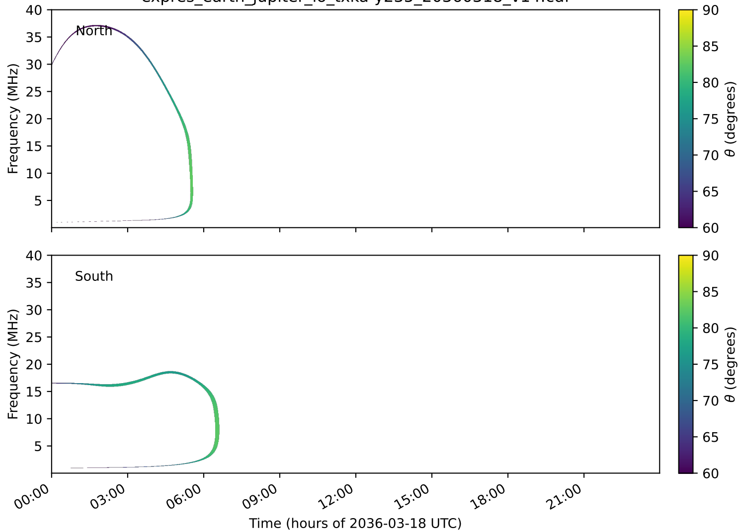
expres_earth_jupiter_io_txka-y235_20360318_v14.cdf
