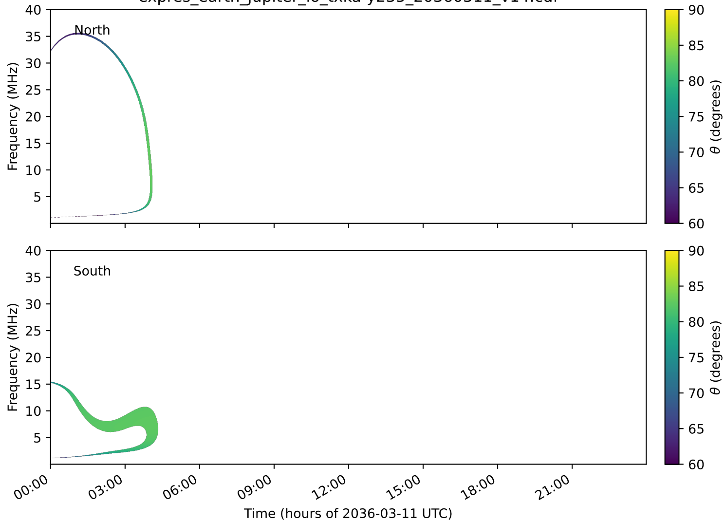
expres_earth_jupiter_io_txka-y235_20360311_v14.cdf
