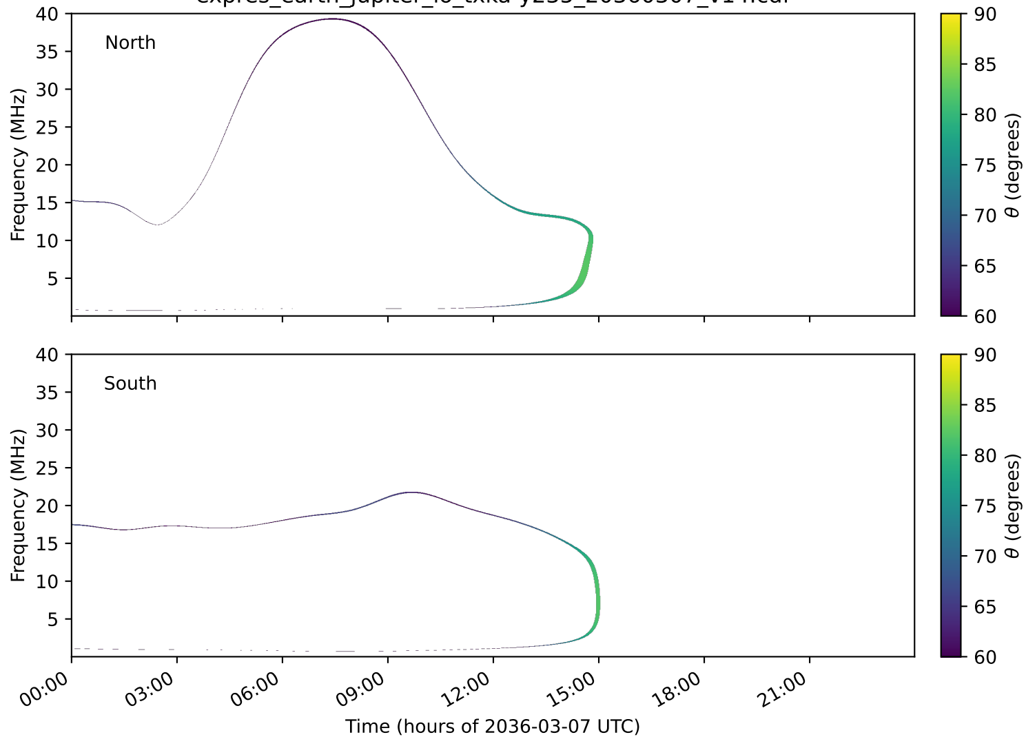
expres_earth_jupiter_io_txka-y235_20360307_v14.cdf
