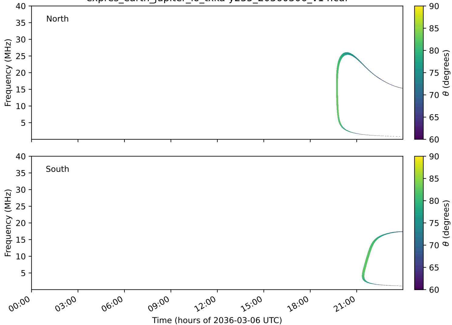
expres_earth_jupiter_io_txka-y235_20360306_v14.cdf
