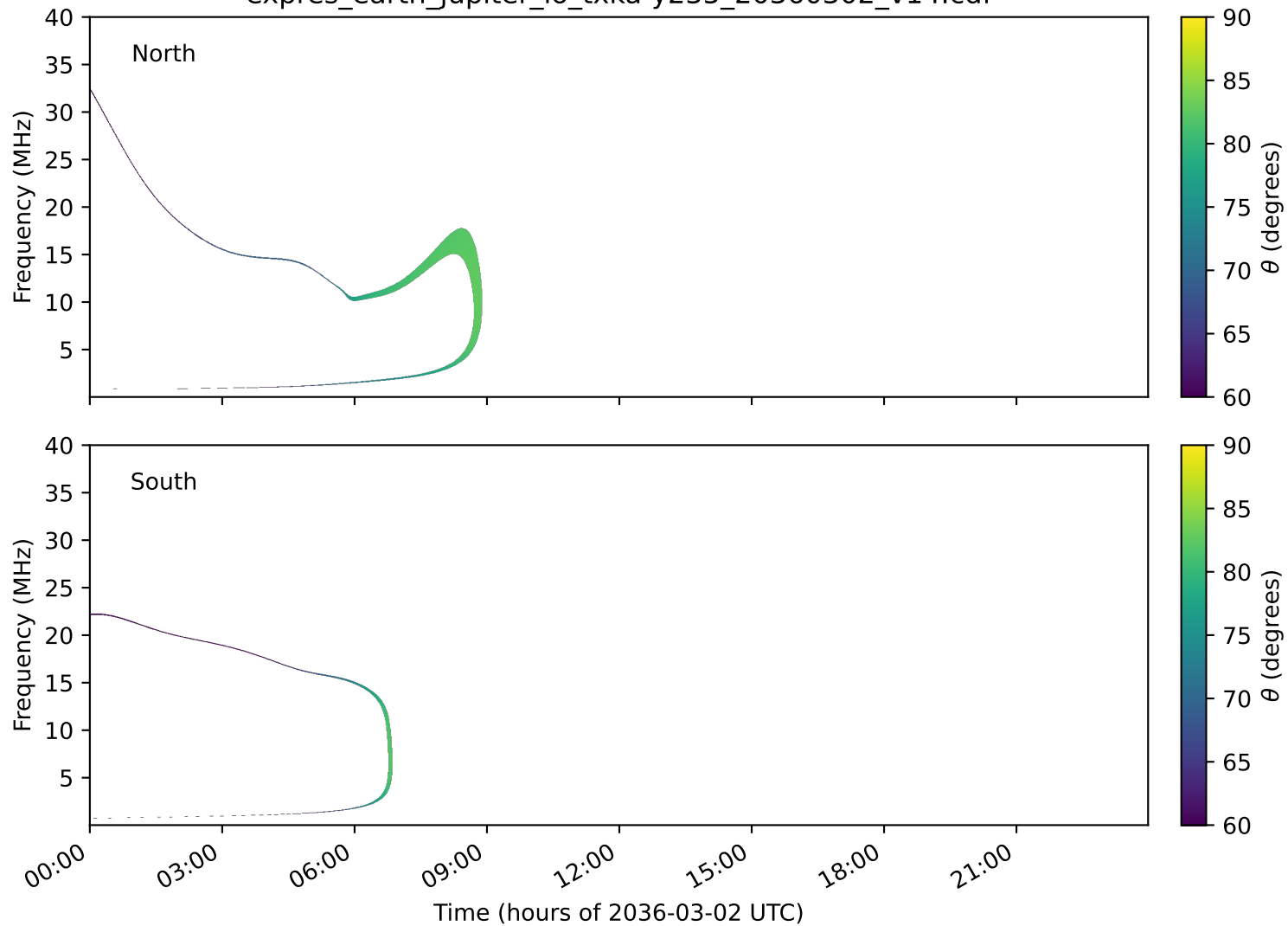
expres_earth_jupiter_io_txka-y235_20360302_v14.cdf
