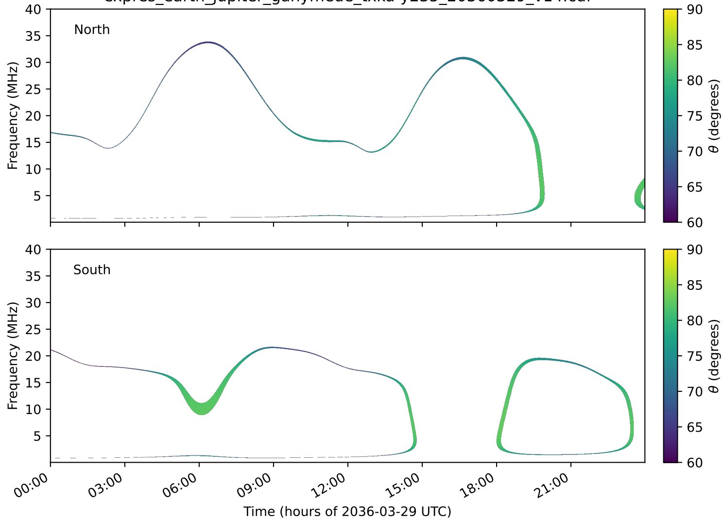
expres_earth_jupiter_ganymede_txka-y235_20360329_v14.cdf
