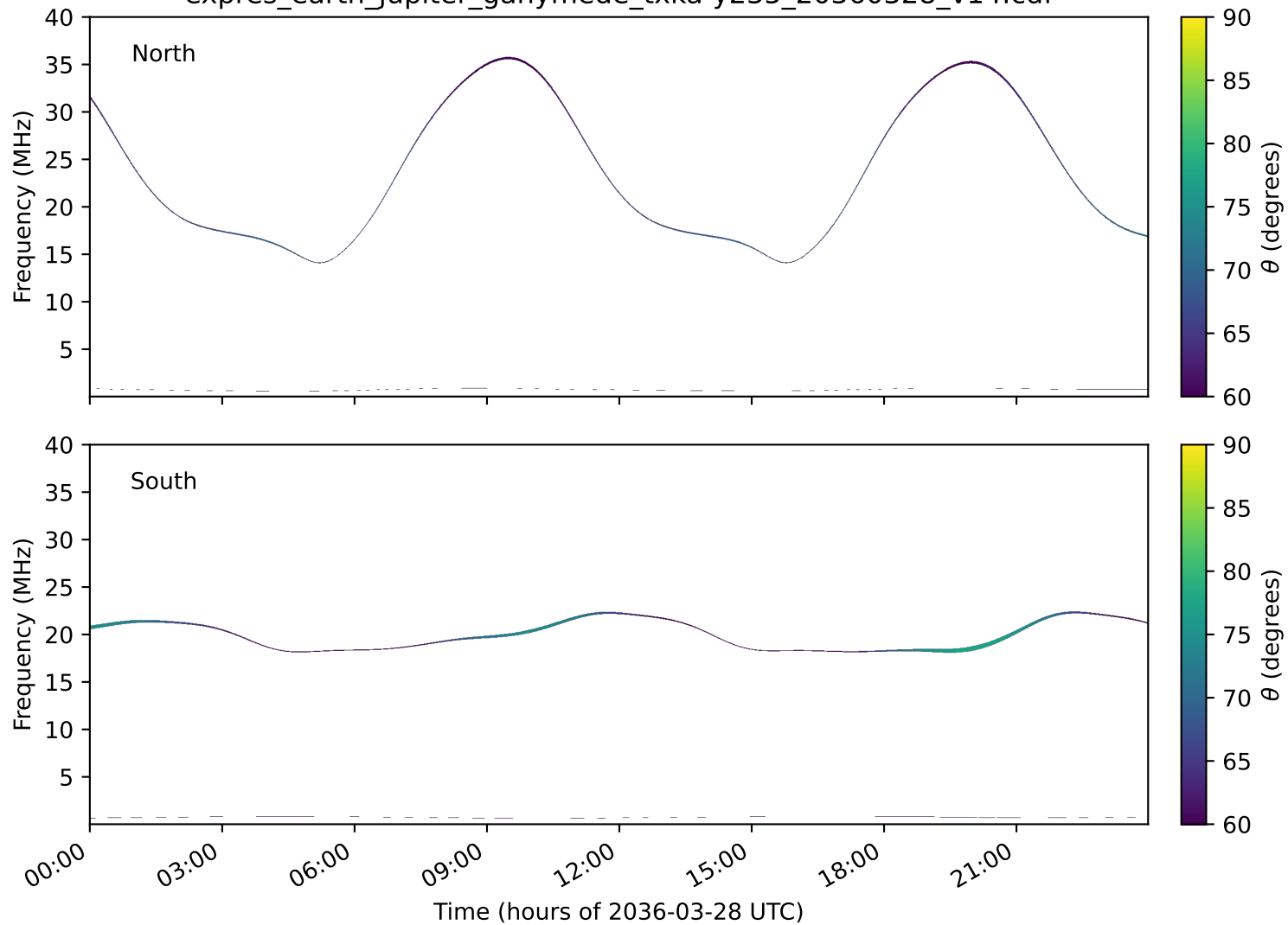
expres_earth_jupiter_ganymede_txka-y235_20360328_v14.cdf
