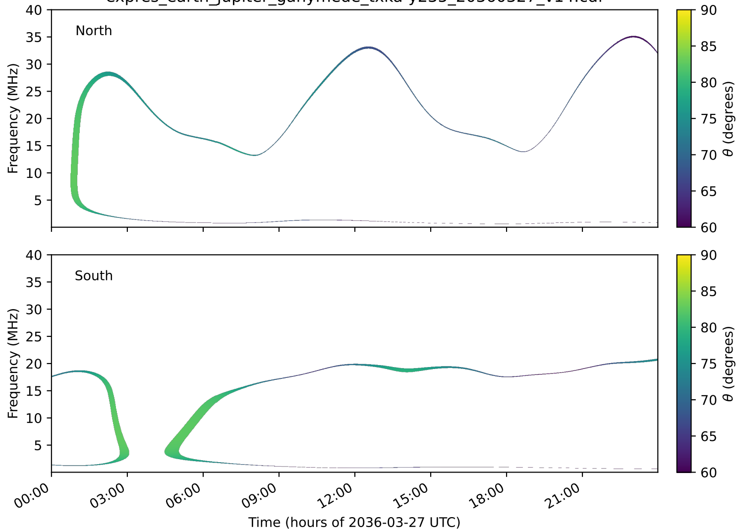
expres_earth_jupiter_ganymede_txka-y235_20360327_v14.cdf
