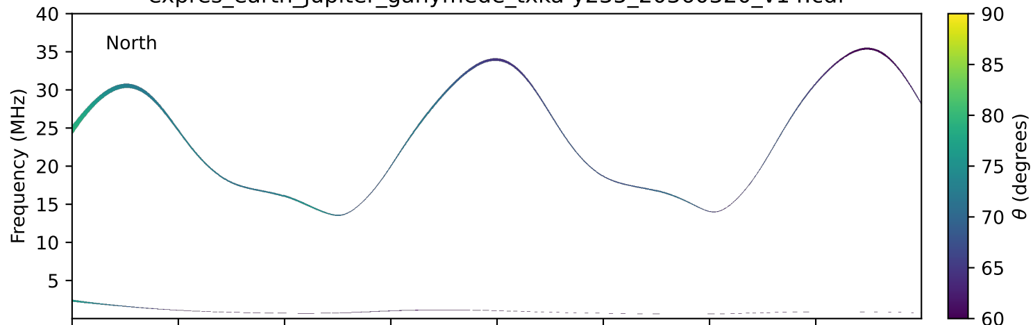
expres_earth_jupiter_ganymede_txka-y235_20360320_v14.cdf
